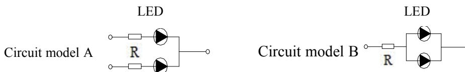
(A)Recommended circuit
